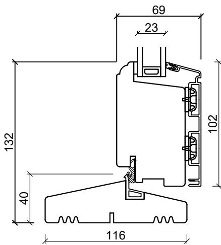
Hardtre Bunnkarm
