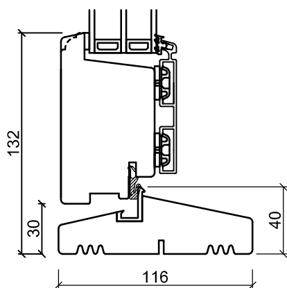
Hardtre Bunnkarm
