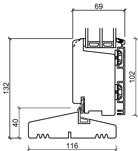
Hardtre Bunnkarm
