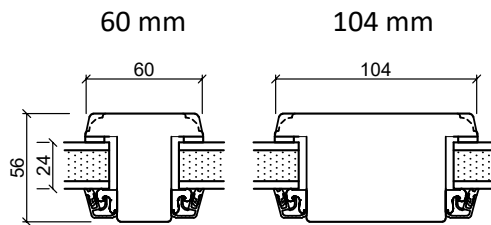
Loddrett post
