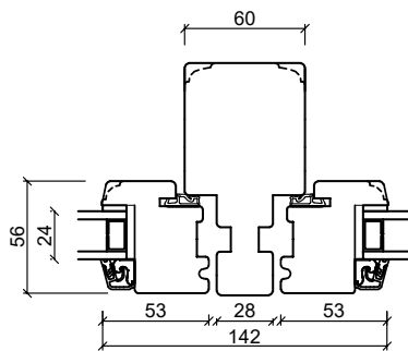
Post
