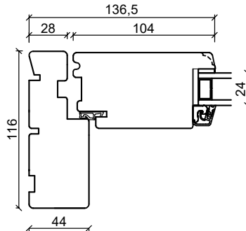
Loddrett post
