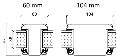
Loddrett post
