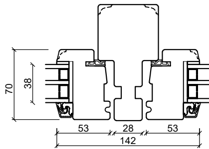
Post
