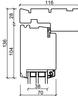
Loddrett post
