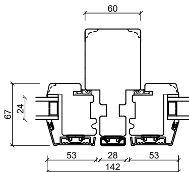
Post
