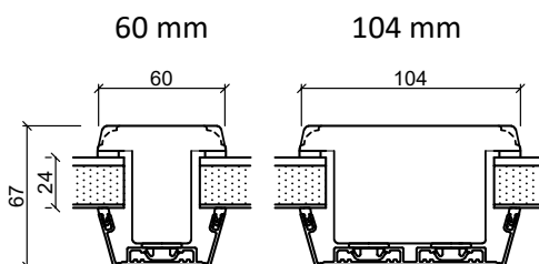
Loddrett post
