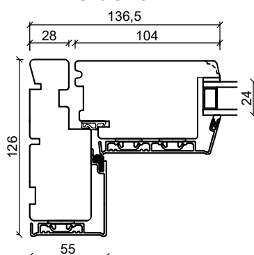
Loddrett post
