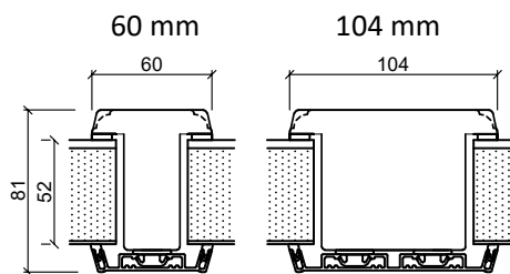
Loddrett post
