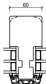
Post
