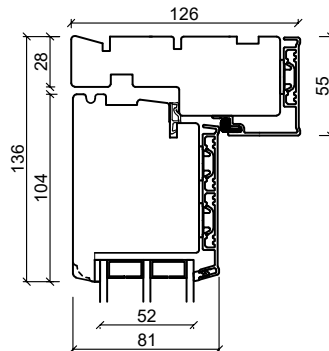
Loddrett post
